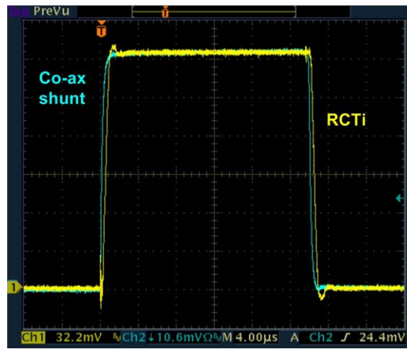
Figure 2. High frequency check Ch1 – RCTi/250A with 1m cable, 700mm coil Ch2 – Co-axial shunt hf(-3dB) 800MHz Time-base 4.0µs/div
