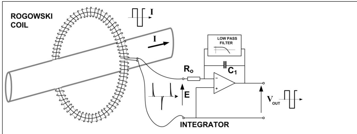
Figure 1. Basic Operation
