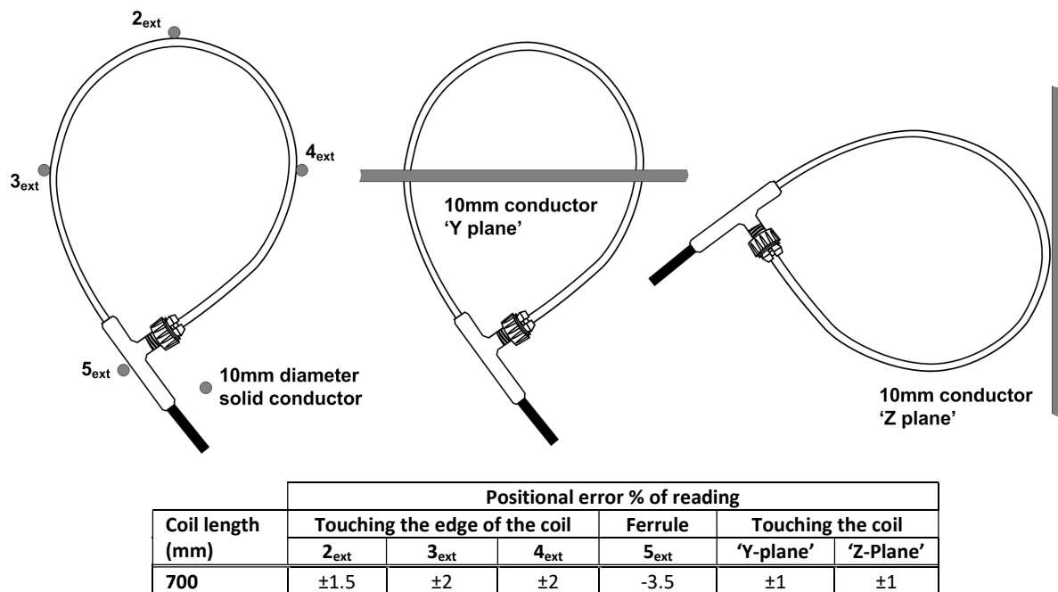
Figure 6. Percentage of external current measured by the RCTi
